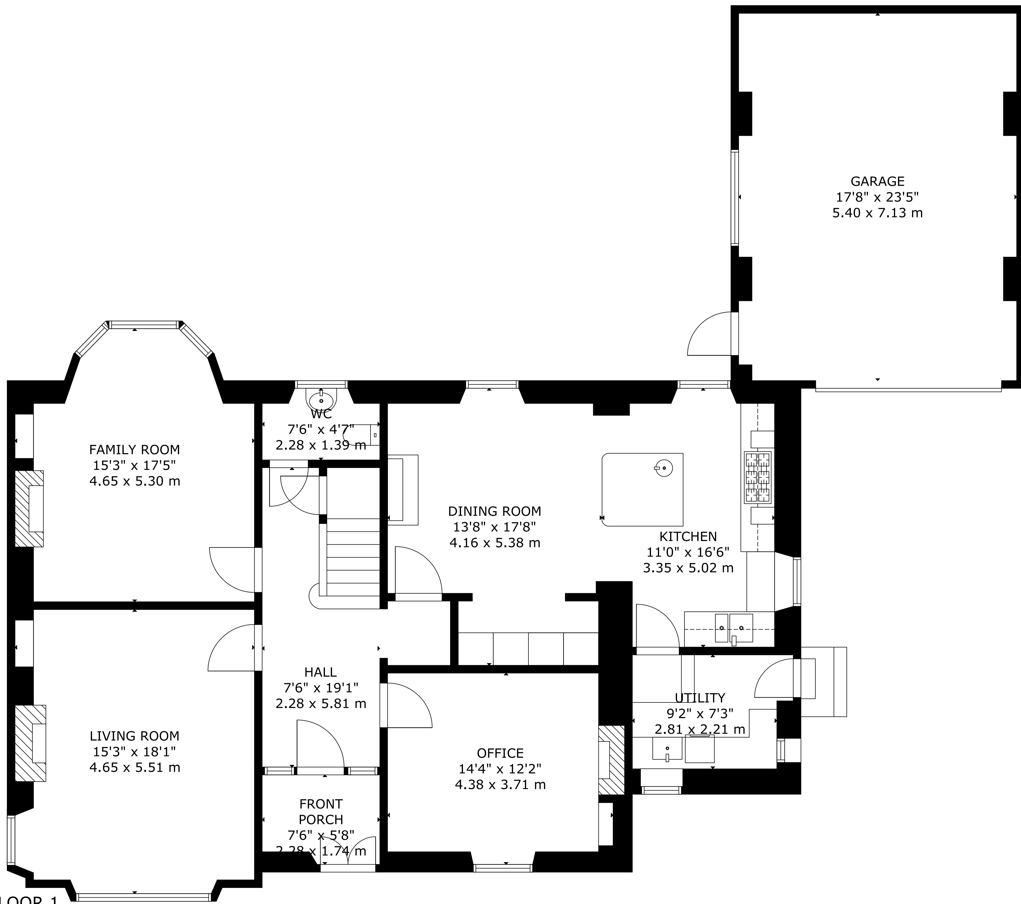
FLOOR 1
