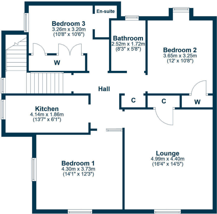
Floor Plan
