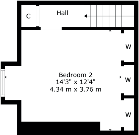
2nd Floor
