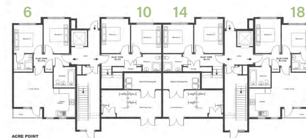
ACRE POINT Block 1 - Ground Floor
